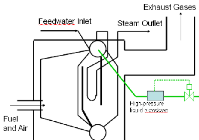
Figura 55: Regulator automat de purjare (Sursa: US DOE ITP Steam BestPractices End User Training Program)
