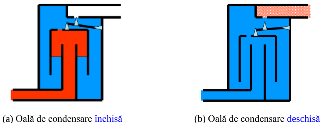
Figura 26: Func ionarea Separatorului  ntr un proces mecanic inversat (Courtesy: US DOE Steam BestPractices End User Training)
