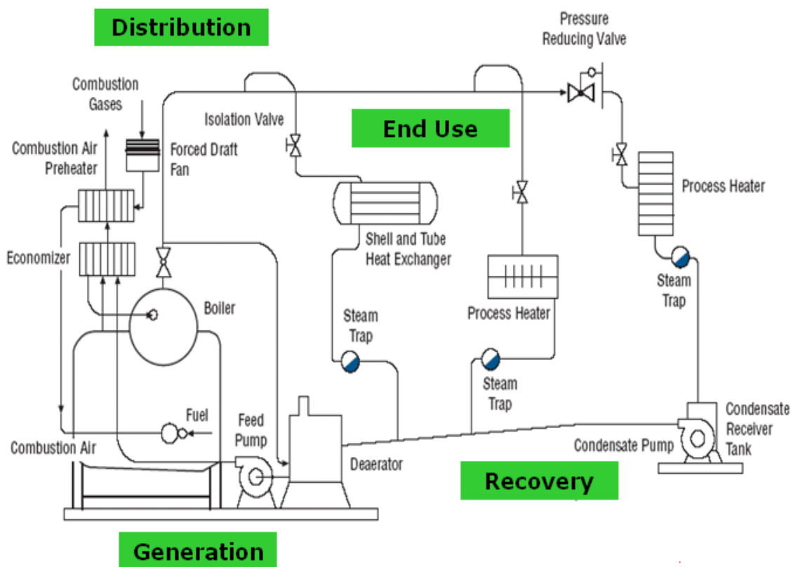
Figure 1: Sistemul general de abur
